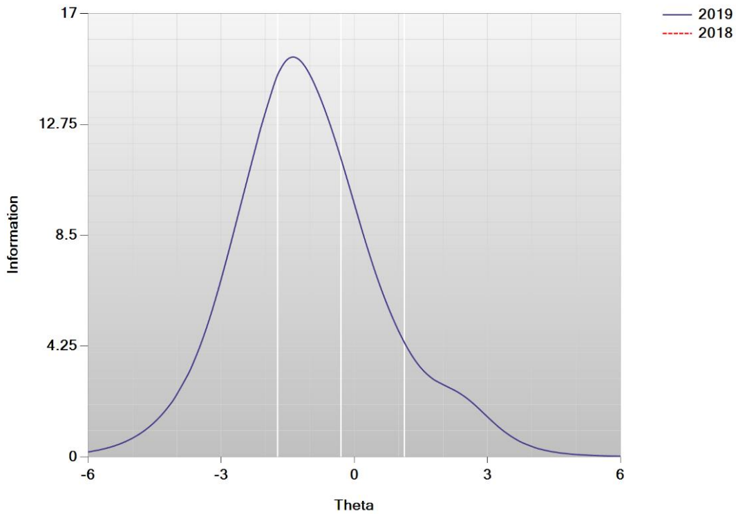
Figure K-14. Test Information Function—ELA Grade 10
