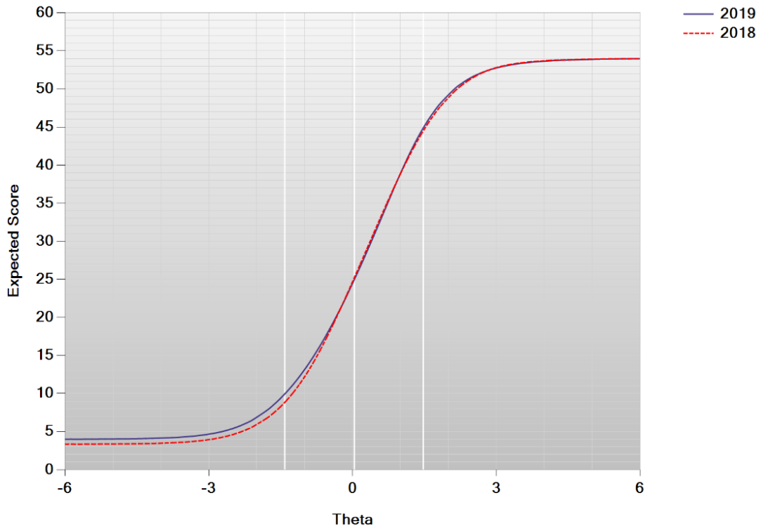
Figure K-23. Test Characteristic Curve—Mathematics Grade 7
