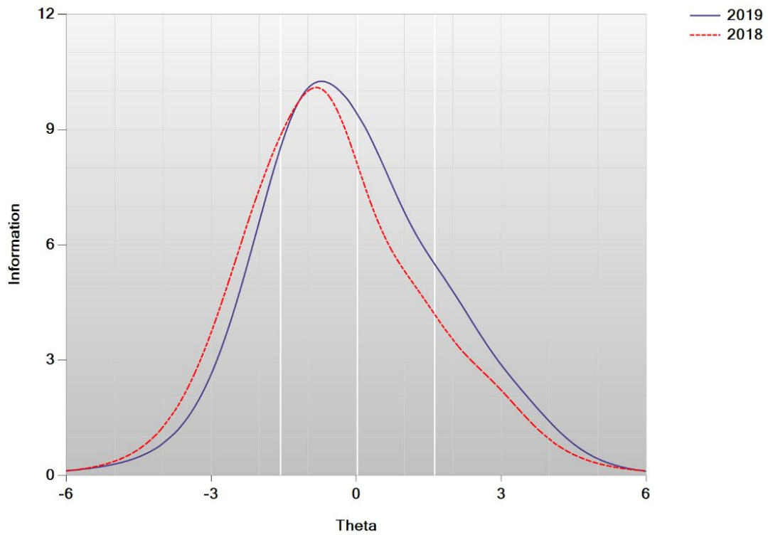
Figure K-4. Test Information Function—ELA Grade 4
