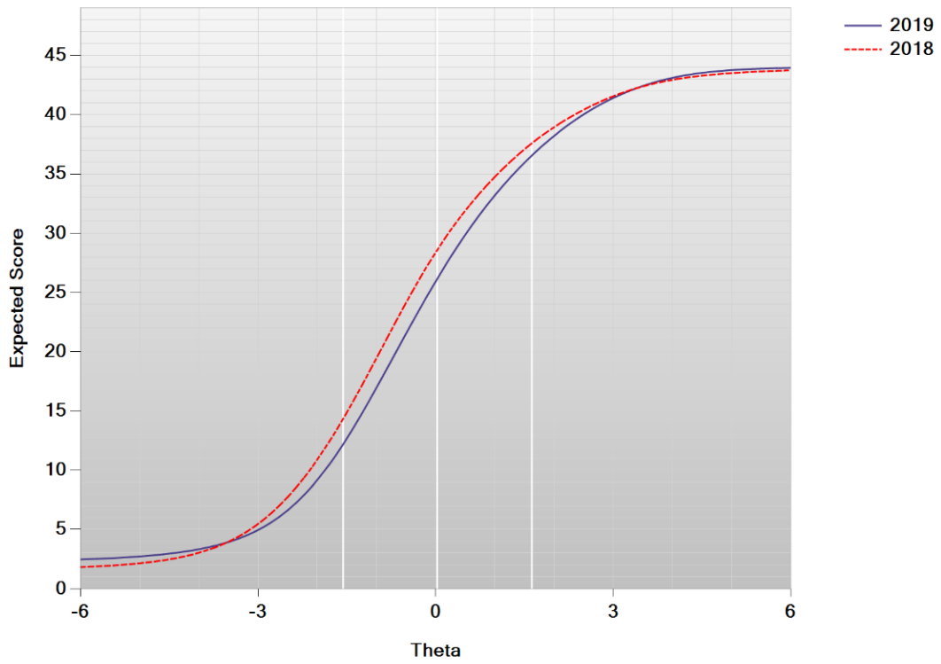
Figure K-3. Test Characteristic Curve—ELA Grade 4
