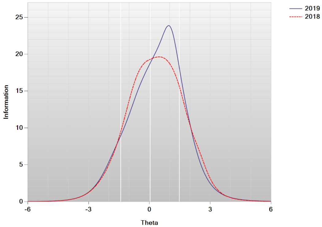
Figure K-24. Test Information Function—Mathematics Grade 7
