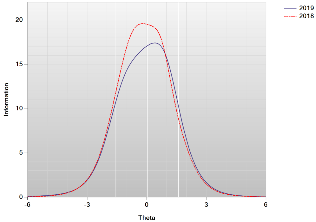
Figure K-20. Test Information Function—Mathematics Grade 5
