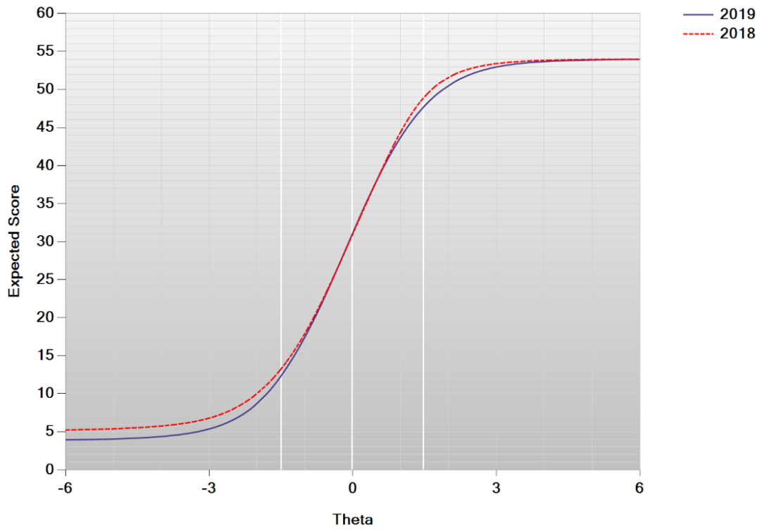
Figure K-25. Test Characteristic Curve—Mathematics Grade 8
