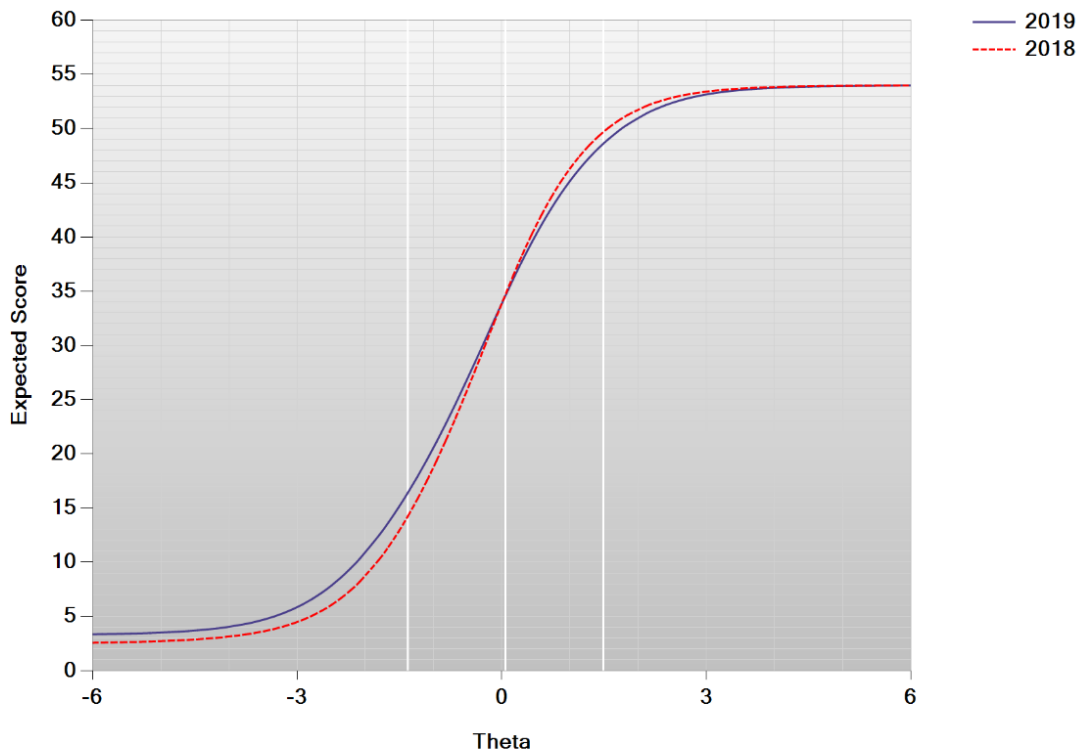
Figure K-17. Test Characteristic Curve—Mathematics Grade 4
