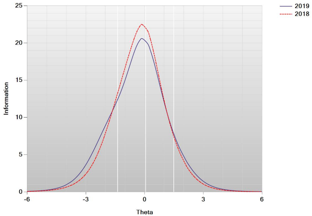
Figure K-18. Test Information Function—Mathematics Grade 4
