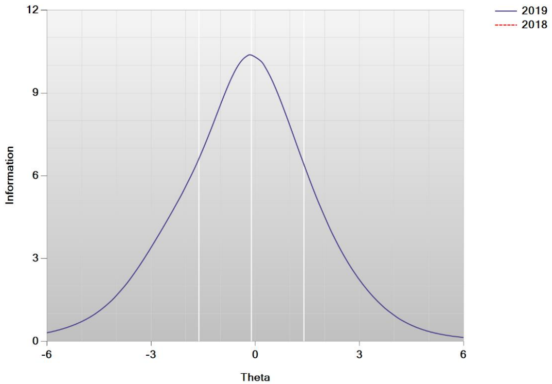
Figure K-30. Test Information Function—STE Grade 5
