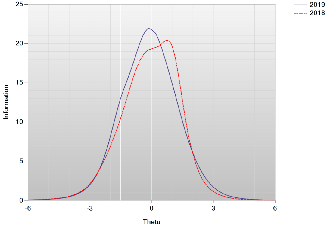
Figure K-26. Test Information Function—Mathematics Grade 8
