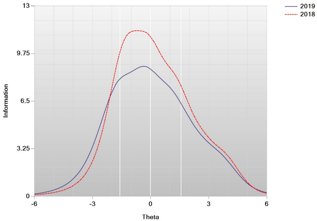
Figure K-8. Test Information Function—ELA Grade 6
