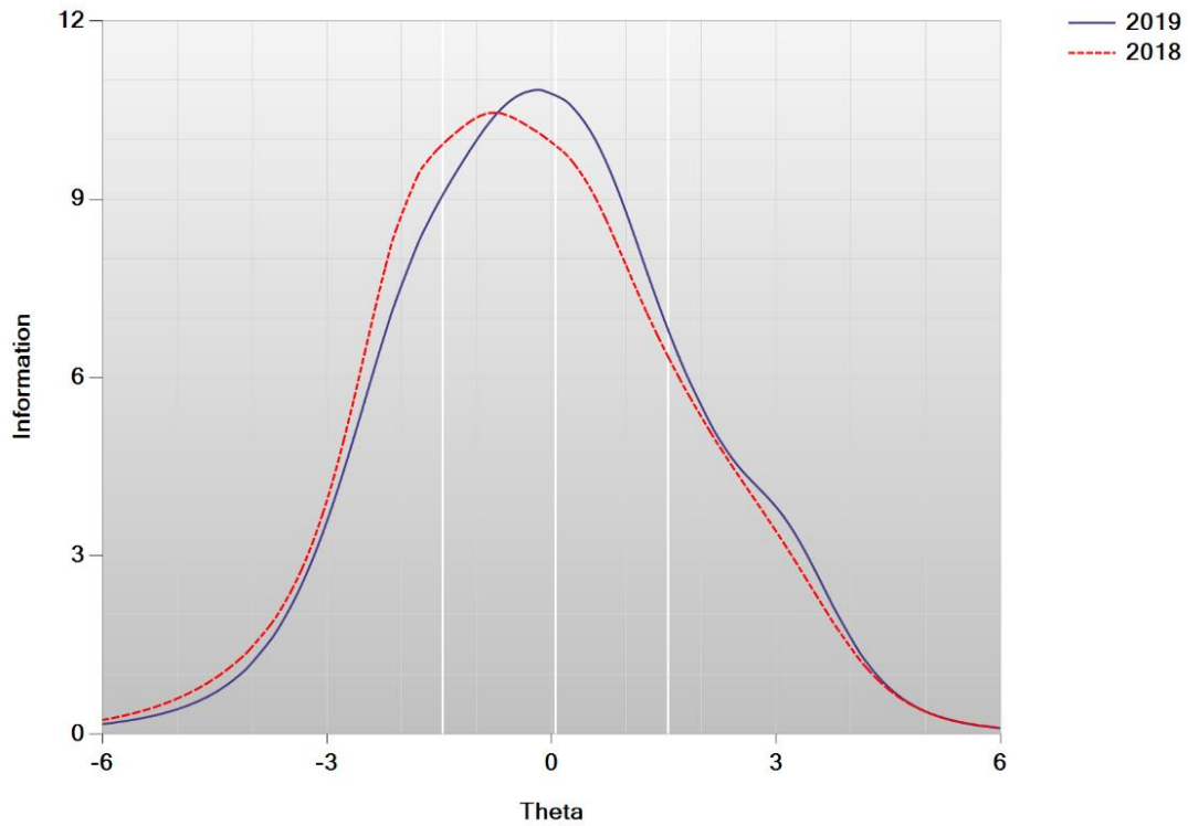
Figure K-12. Test Information Function—ELA Grade 8
