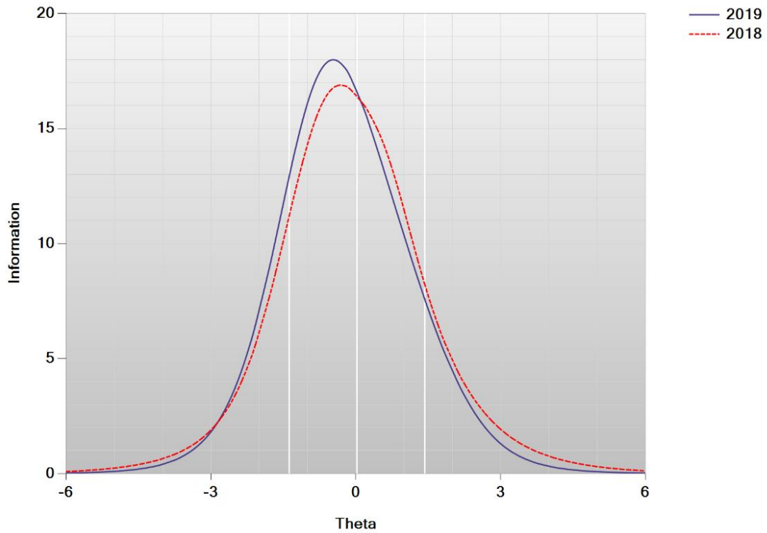
Figure K-16. Test Information Function—Mathematics Grade 3
