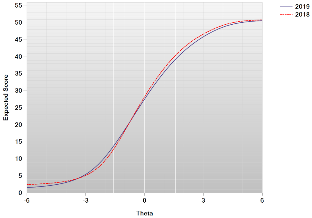
Figure K-7. Test Characteristic Curve—ELA Grade 6
