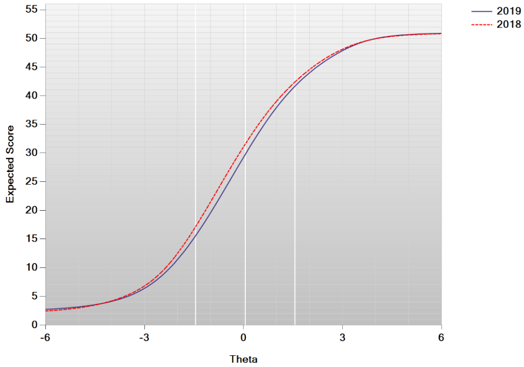
Figure K-11. Test Characteristic Curve—ELA Grade 8
