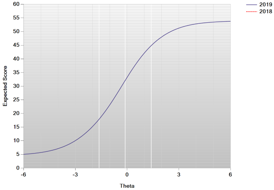
Figure K-29. Test Characteristic Curve—STE Grade5
