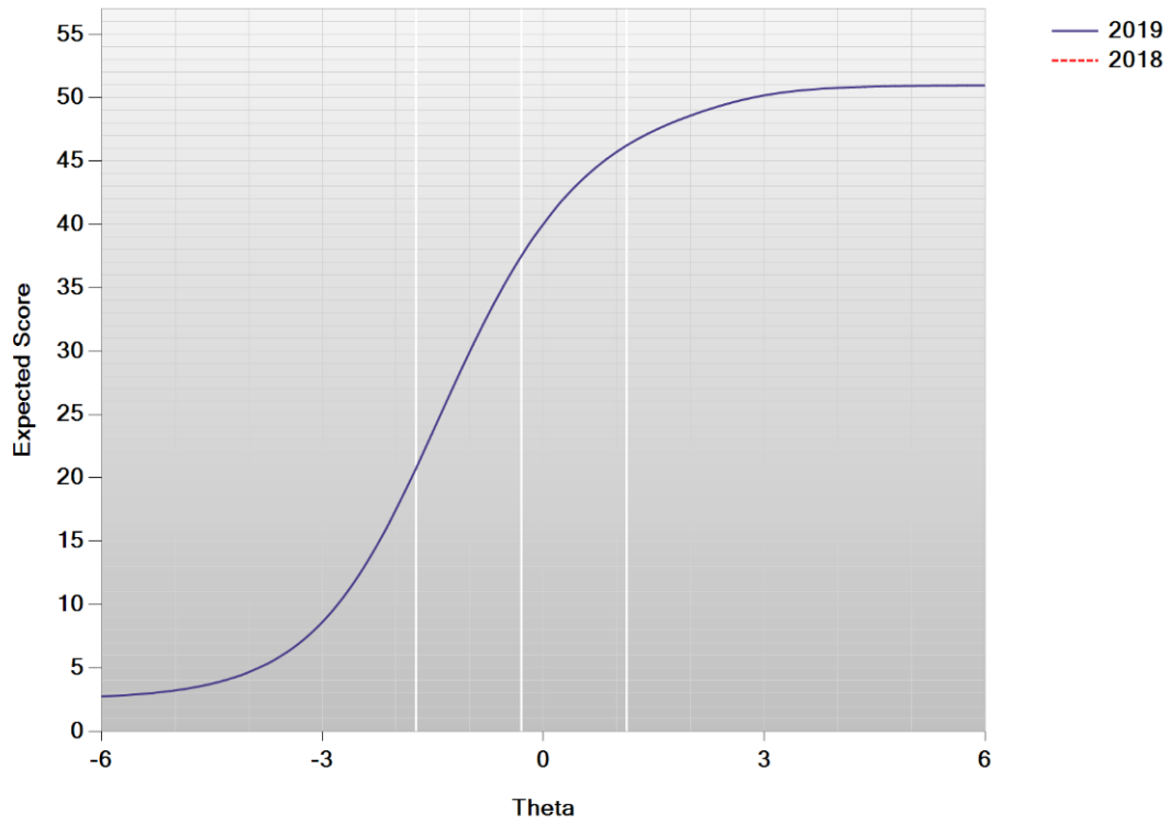
Figure K-13. Test Characteristic Curve—ELA Grade 10
